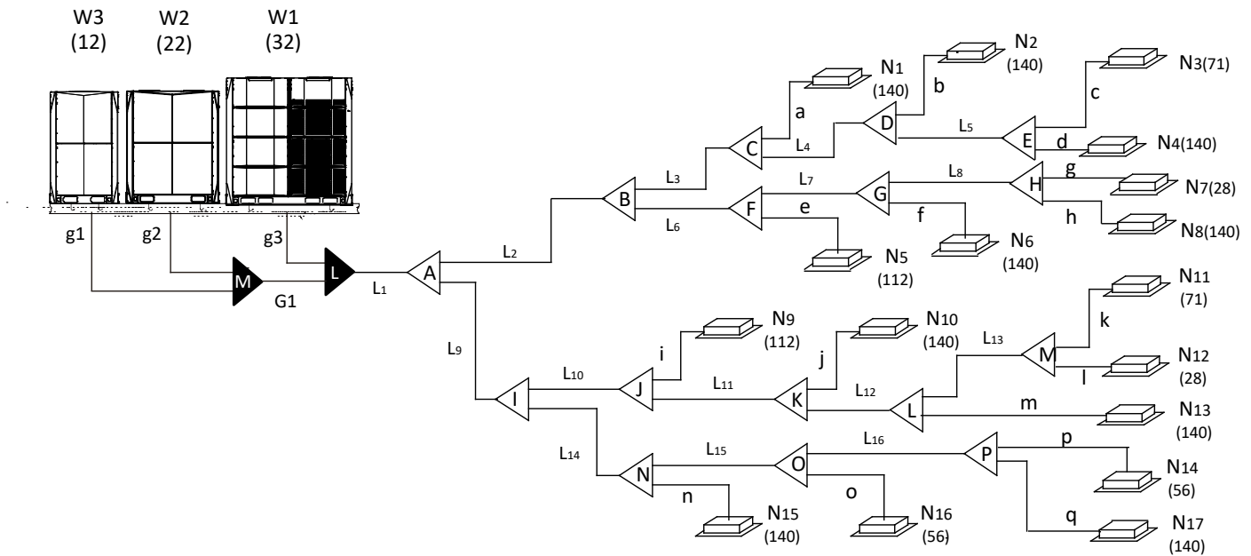
Figure 3-4.3: Selecting piping diameters
