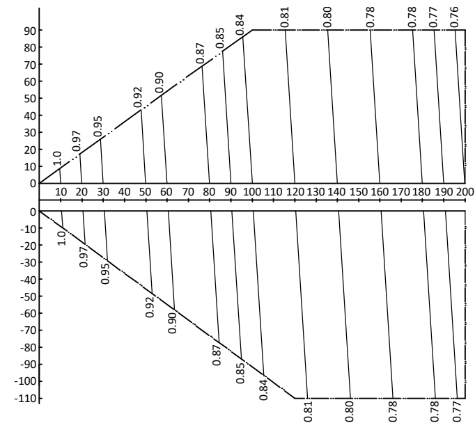
Figure 2-8.1: Rate of change in cooling capacity
