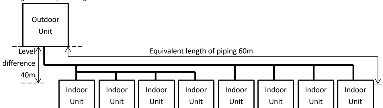
Figure 1-6.2: System diagram
